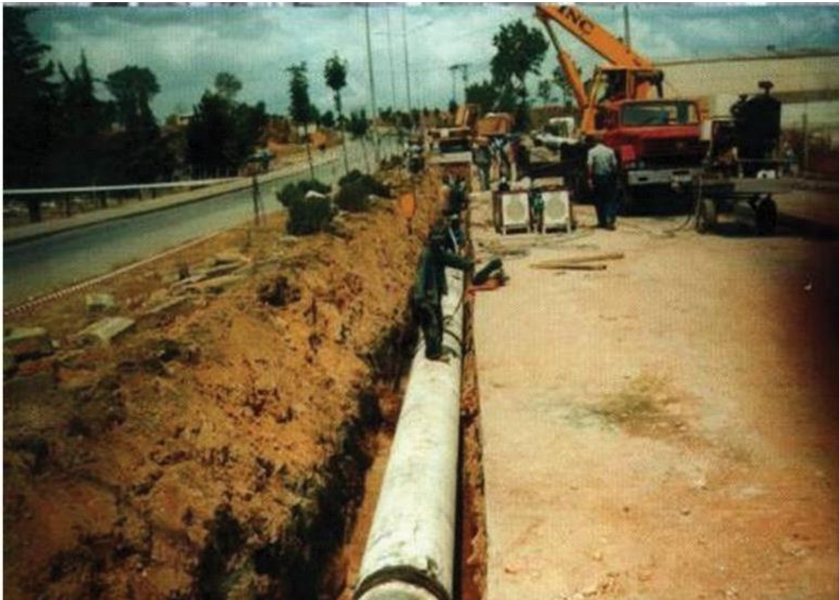
PIPELINE LAYING
